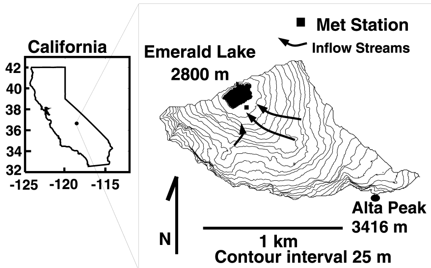
Figure 4. Location and topographic map of the Emerald lake watershed.
