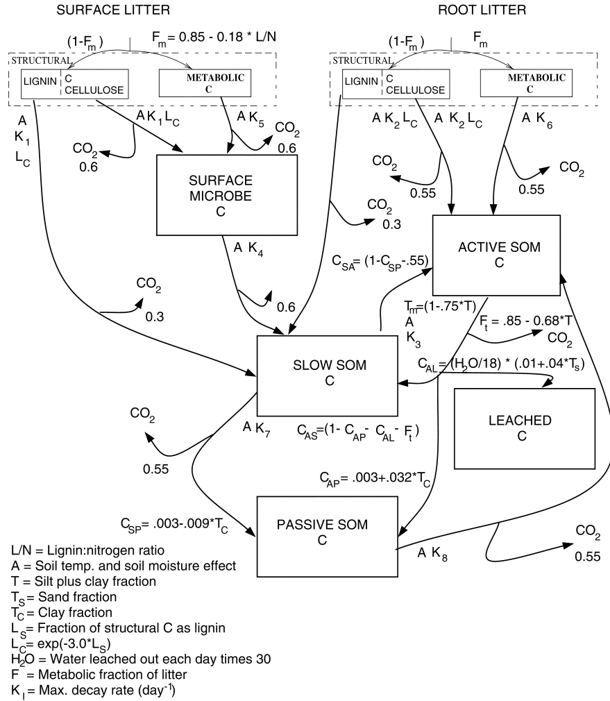
Figure 1. Carbon box diagram (Parton et al. 1993)
